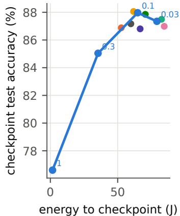
UCI HAR, \phi = 0.25
