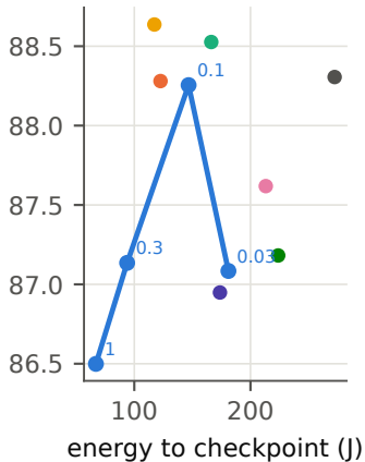
UCI HAR, \phi = 1.0
