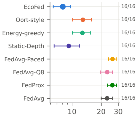
UCI HAR, \phi = 0.25
