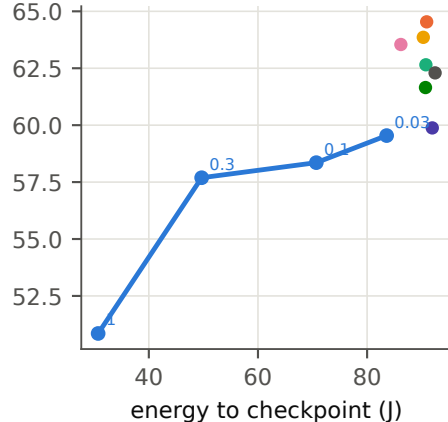
Speech Commands, \phi = 1.0
