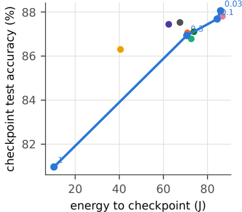
UCI HAR, \phi = 1.0
