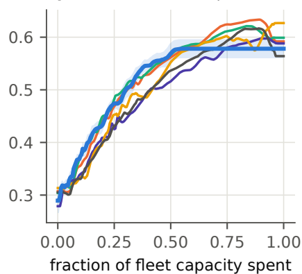
Speech Commands, \phi = 1.0
