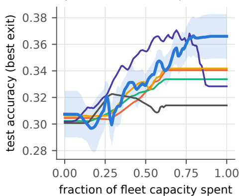
Speech Commands, \phi = 0.1
