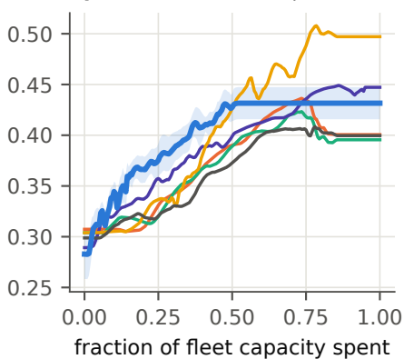
Speech Commands, \phi = 0.25
