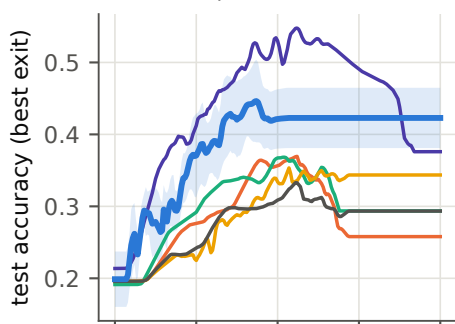
Speech Commands, \phi = 0.1
