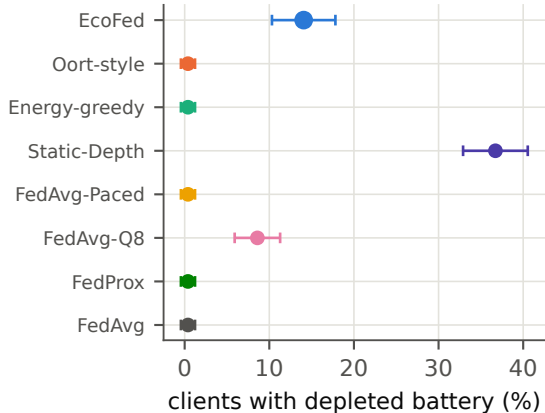
UCI HAR, \phi = 0.25
