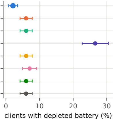
Speech Commands, \phi = 0.25
