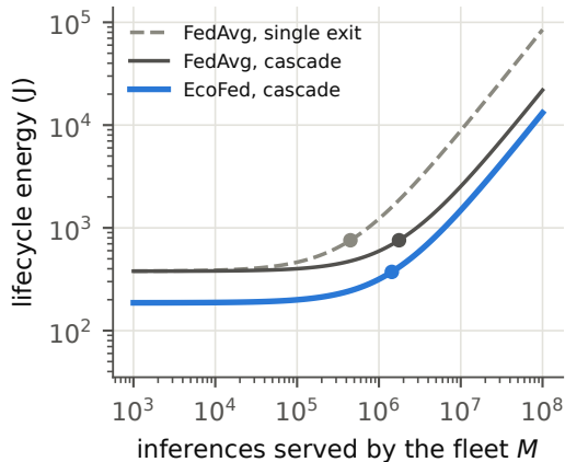
UCI HAR, \phi = 1
