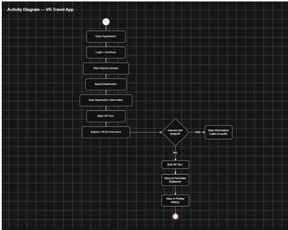
Figure 2.22: Activity Diagram for Destination Exploration and VR Tour Session
