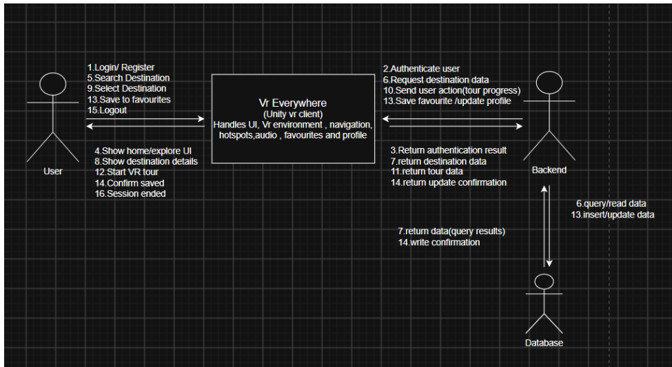
Figure 2.24: Collaboration Diagram of VR Everywhere System Components
