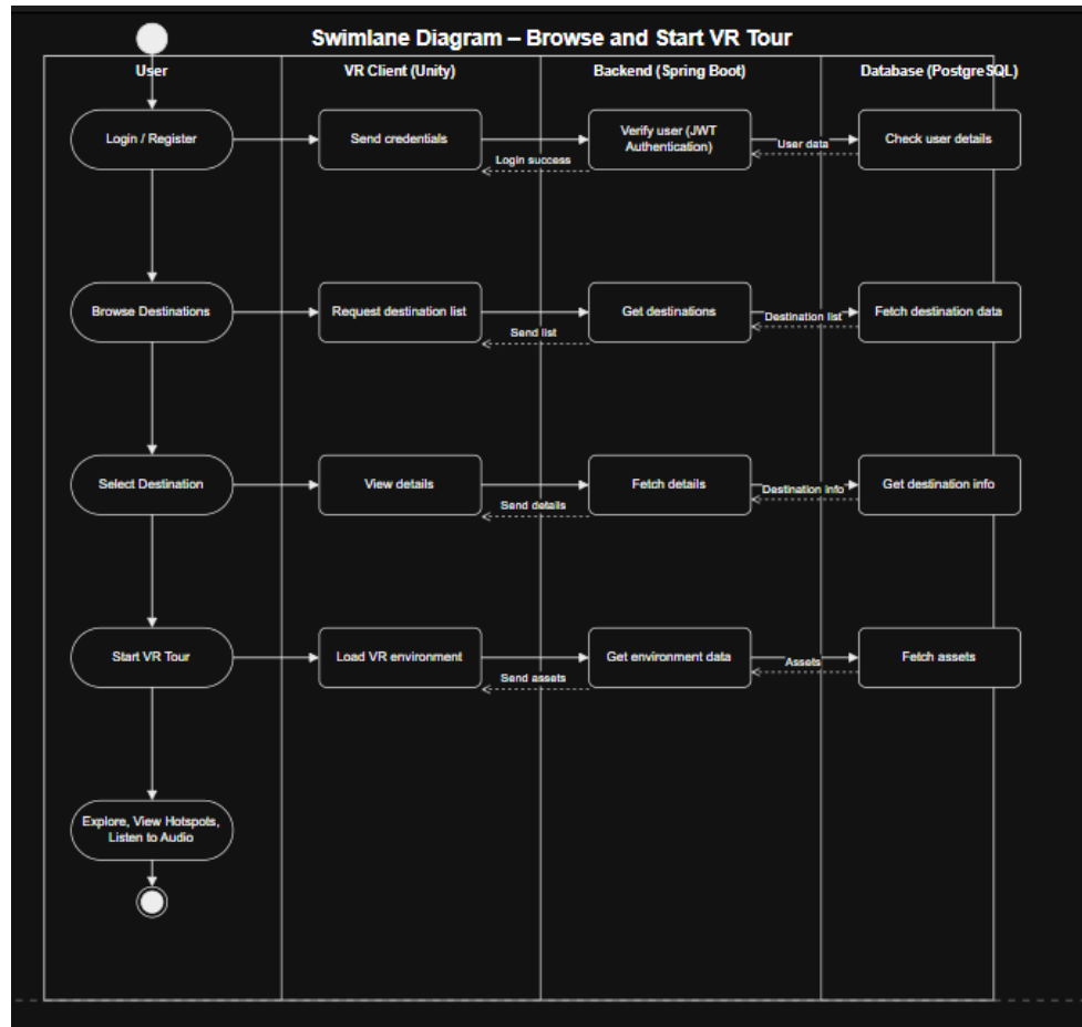
Figure 2.25: Swimlane Diagram for User, VR Client, Backend API, and Database Workflow
