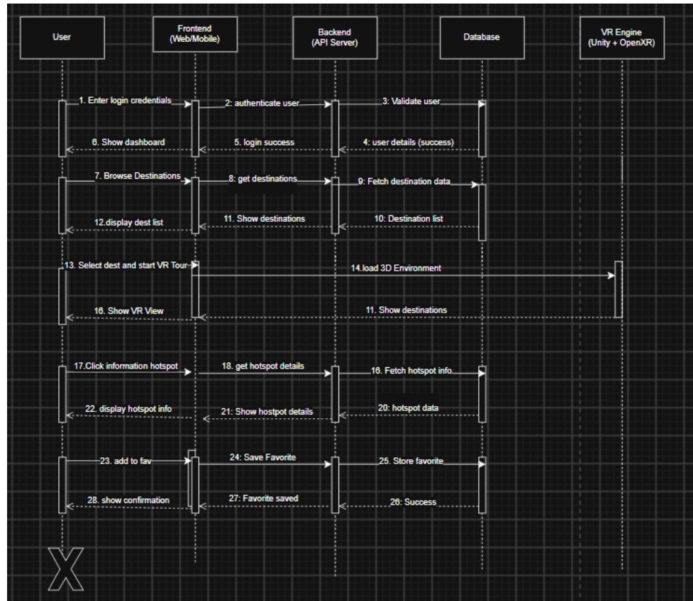
Figure 2.23: Sequence Diagram for Authentication, Scene Loading, and Hotspot Interaction
