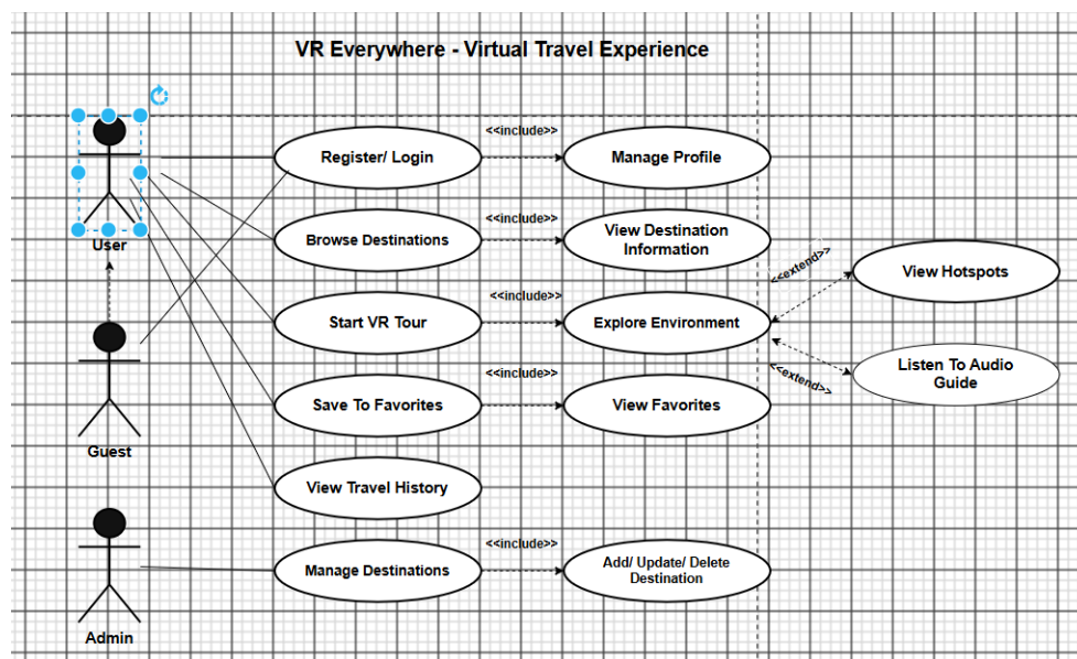
Figure 2.7: Use Case Diagram of VR Everywhere Platform
