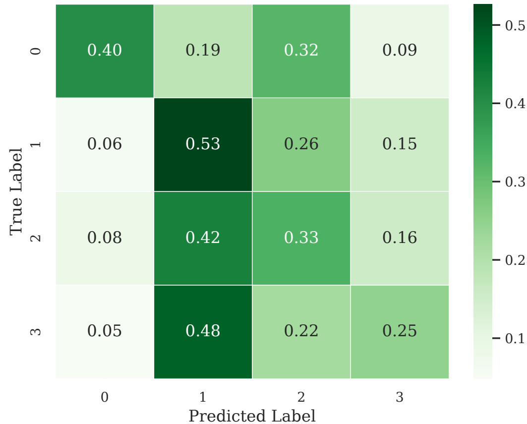
MLP (Normalized)
