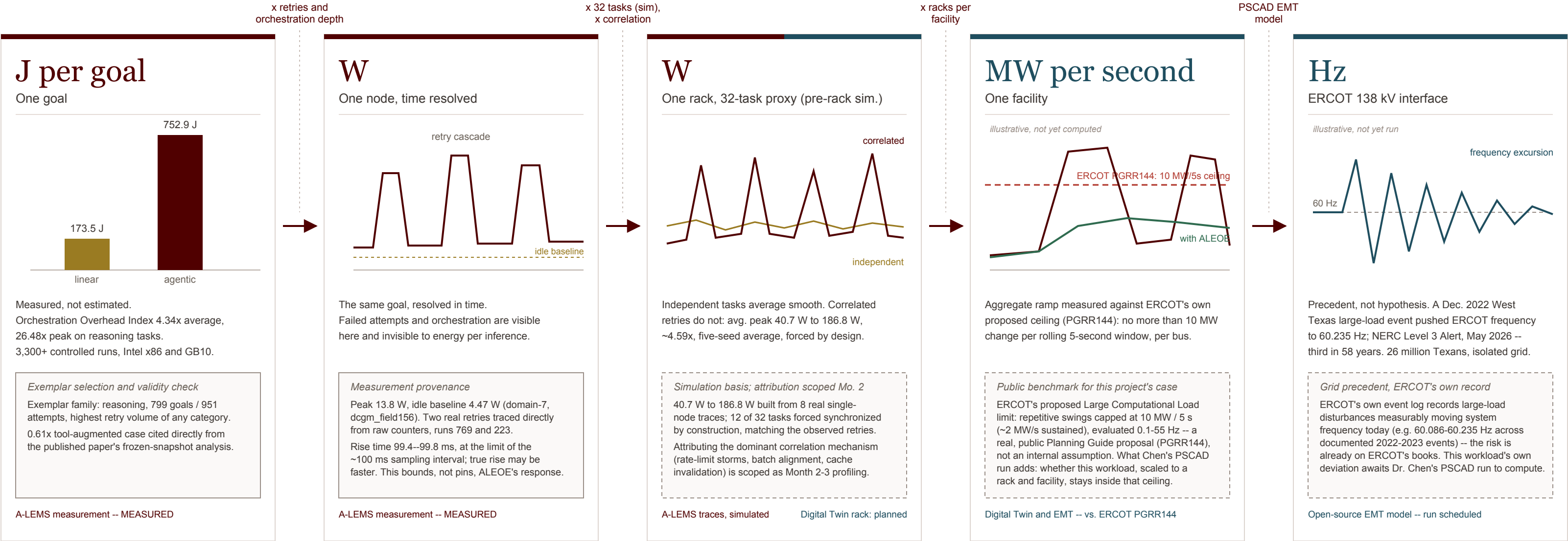
Figure 2, chip to grid. Every arrow changes the unit. Solid boxes are measured, simulated, or externally cited; dashed boxes are scoped as funded next-phase work.
