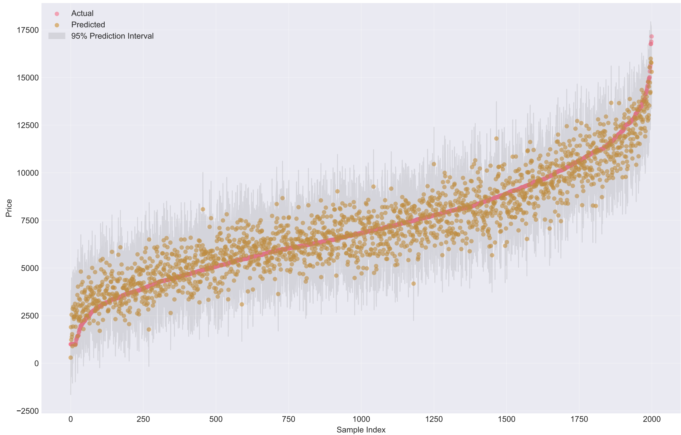
Prediction Intervals
