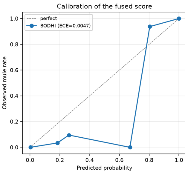
Fig. 2. Calibration of the fused score (ECE 0.0047). The score has to mean what it says before it can drive an automated kill-switch.
