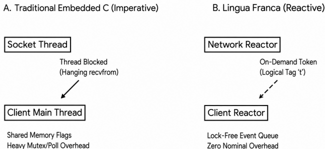
Figure 4: Architectural Comparison of Fault Signaling
