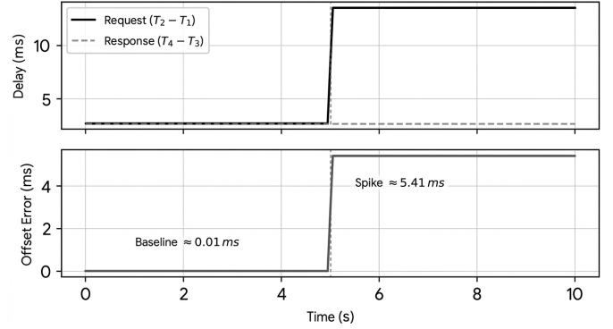
Figure 3: NTP Fluctuations under Congestion Asymmetry
