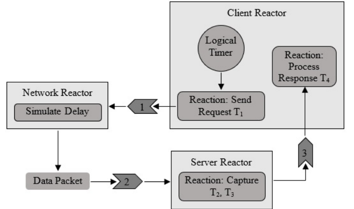
Figure 2: Reactive (LF) Event Graph
