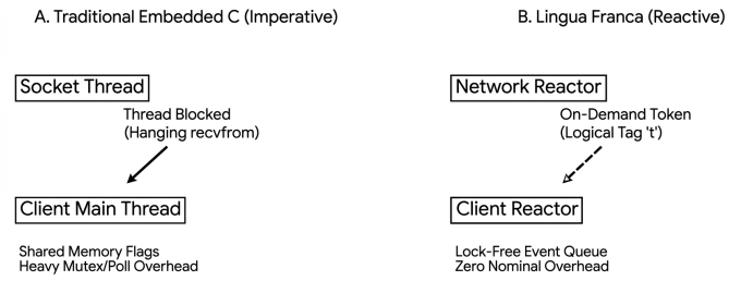
Figure 4: Architectural Comparison of Fault Signaling
