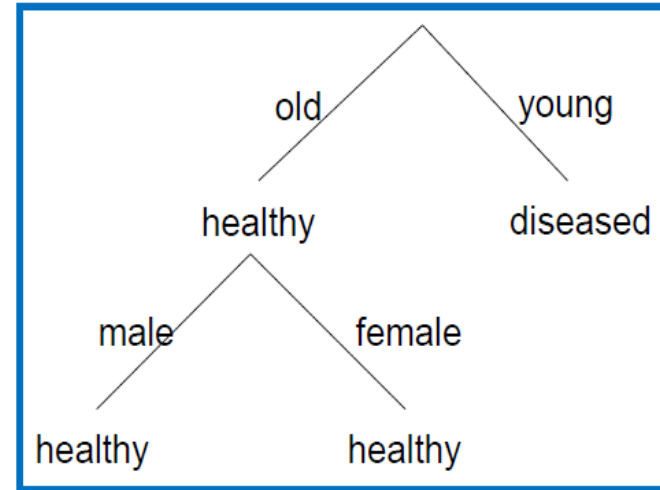
Tree 2
