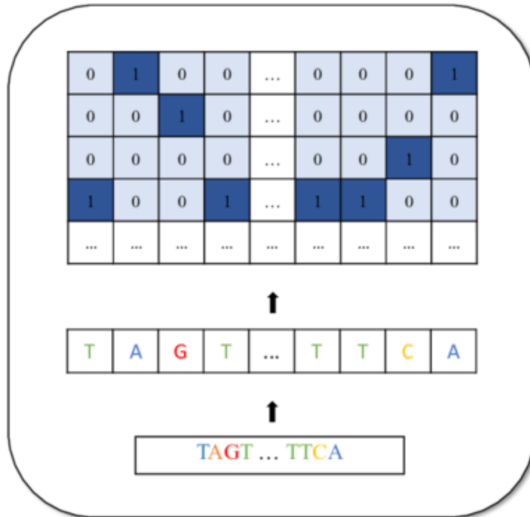
One-hot encoding
