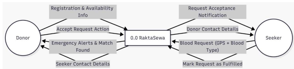
Figure 6 DFD Level 0
