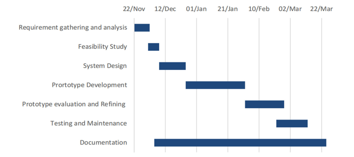
Figure 4 Gantt Chart
