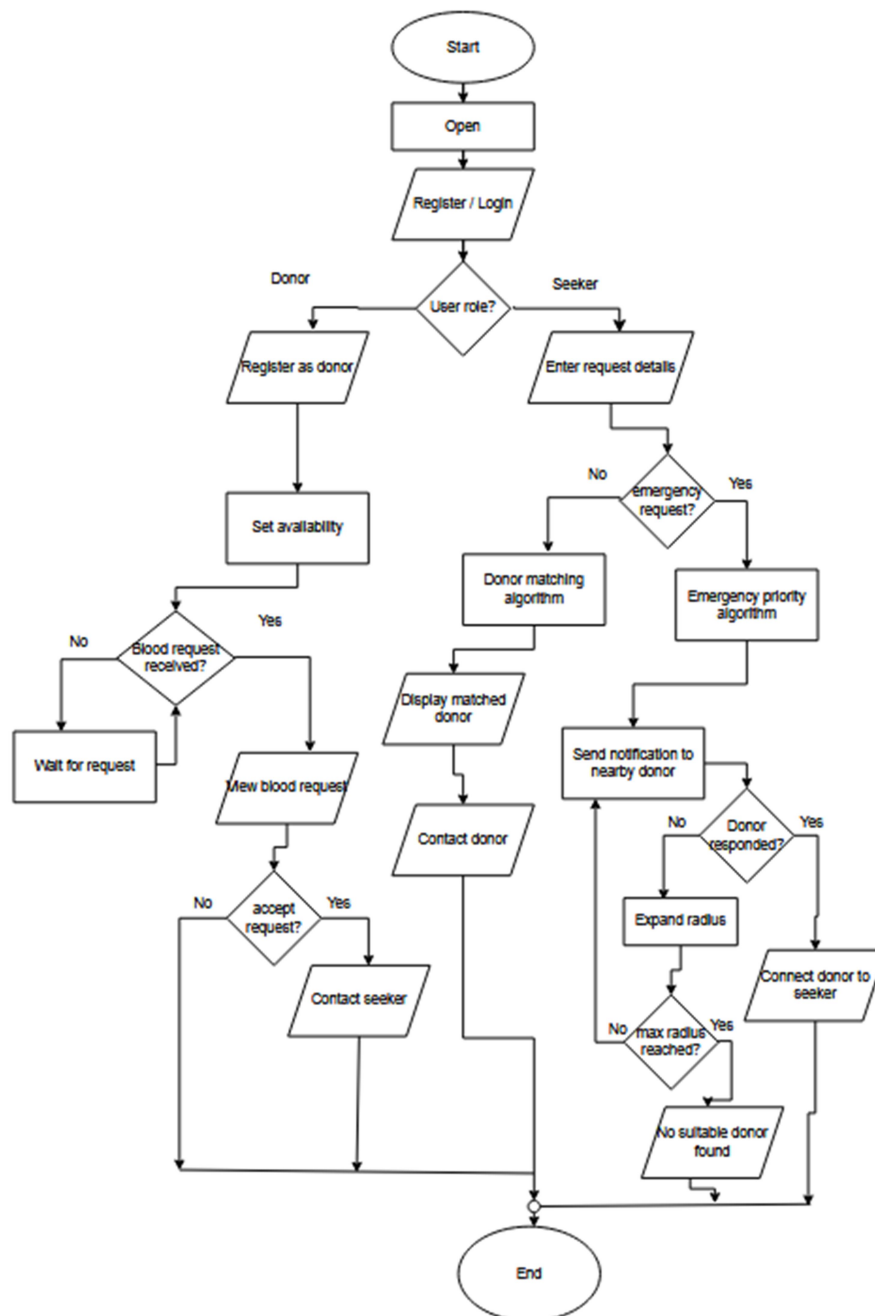
Figure 3 System flow chart
