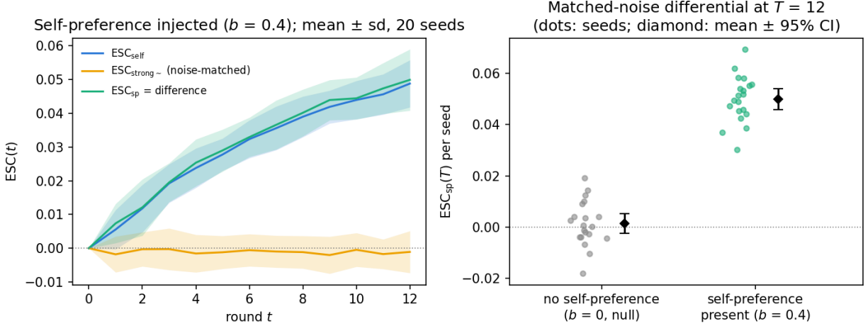
Figure 2: Left — ESC_{self} , noise-matched ESC_{strong \sim} , and their difference ESC_{sp} under injected self-preference ( b = 0.4 ). Right — ESC_{sp}(T) seed cloud under null ( b = 0 ) vs. preference present.
