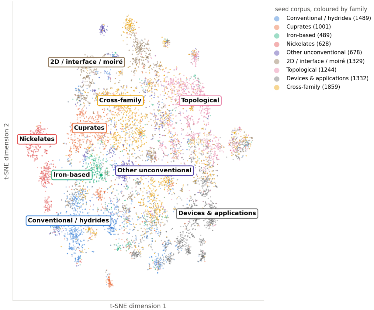
Figure 2: Semantic map of the seed corpus (TF-IDF, truncated SVD, t-SNE), coloured by material family. Each family is labelled at its density peak, with a leader line where the label had to be moved to avoid a collision; nine categorical hues cannot be told apart reliably, so the labels rather than the colours carry identity. Per-family counts match Table 1.
