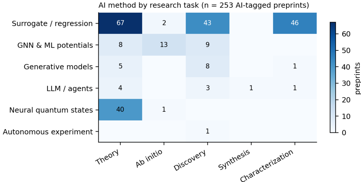
Figure 4: AI-method usage by mode of inquiry across the working corpus. Synthesis carries a single record, and it comes from the supplement: the systematic seed has none. The figure combines 120 seed records with 133 from the targeted supplement, so 53% of it was retrieved by keyword rather than sampled systematically. It therefore describes the AI-for-superconductivity literature this survey assembled, not an adoption rate; the rate is the seed-only 1.2% quoted above.
