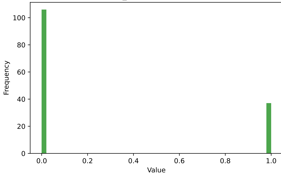
y_train Distribution
