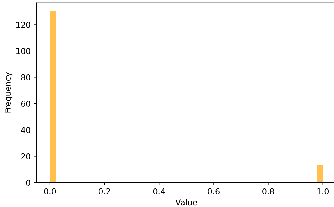
y_test Distribution
