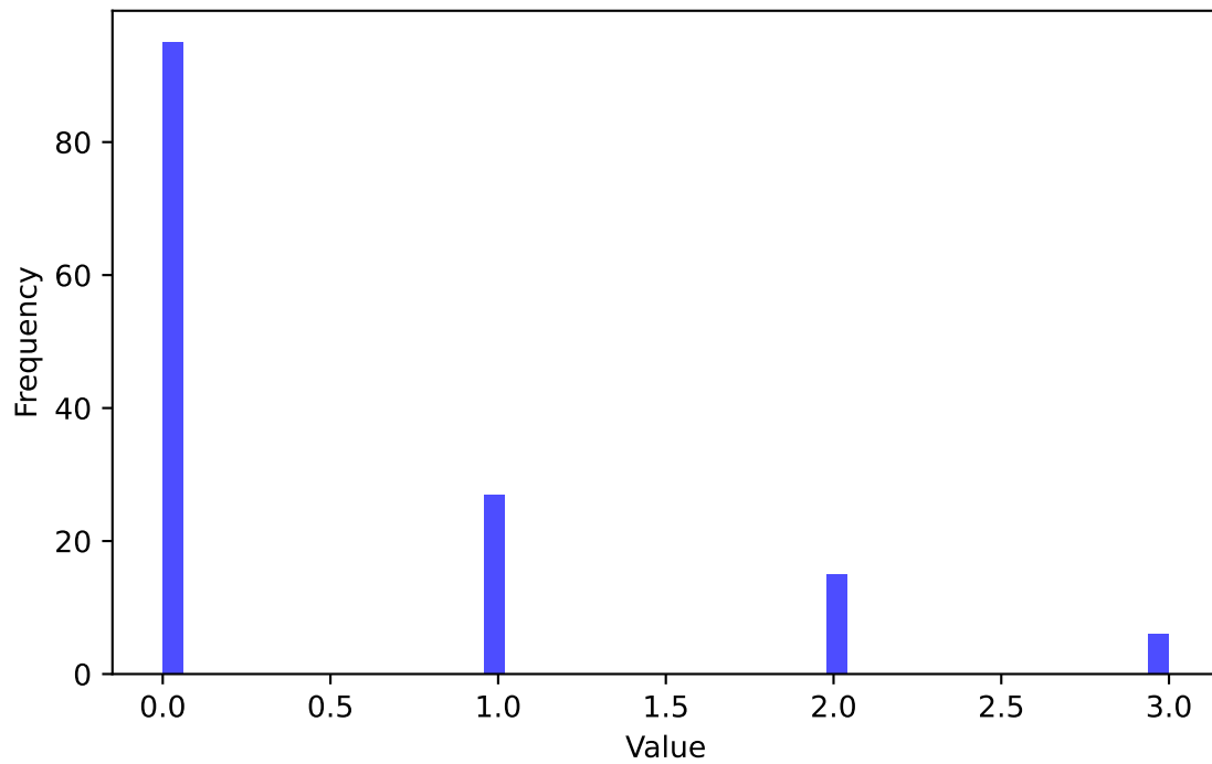
y_train Distribution
