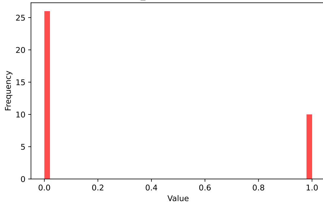
y_test Distribution
