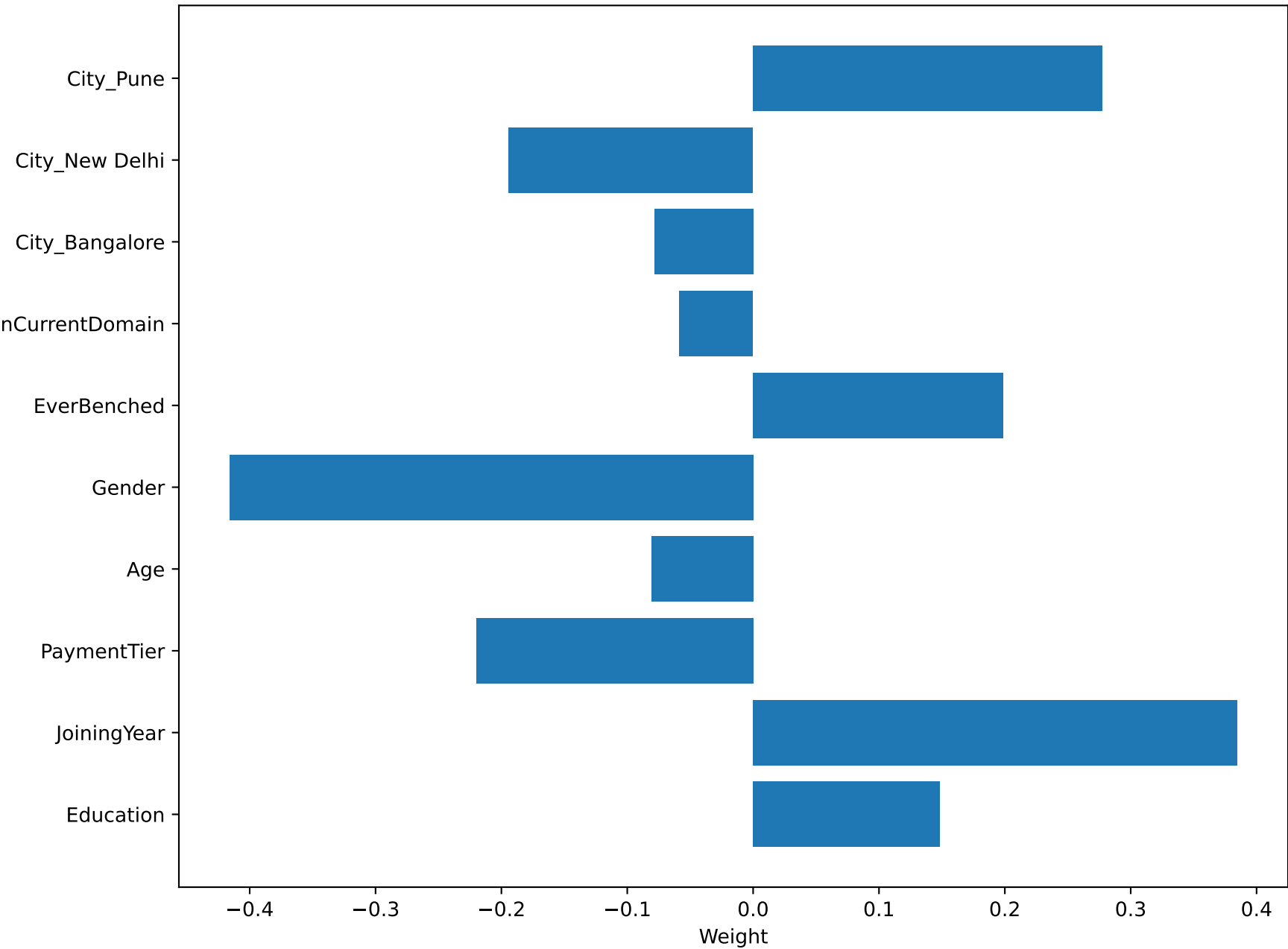
Logistic Regression Model Weights
