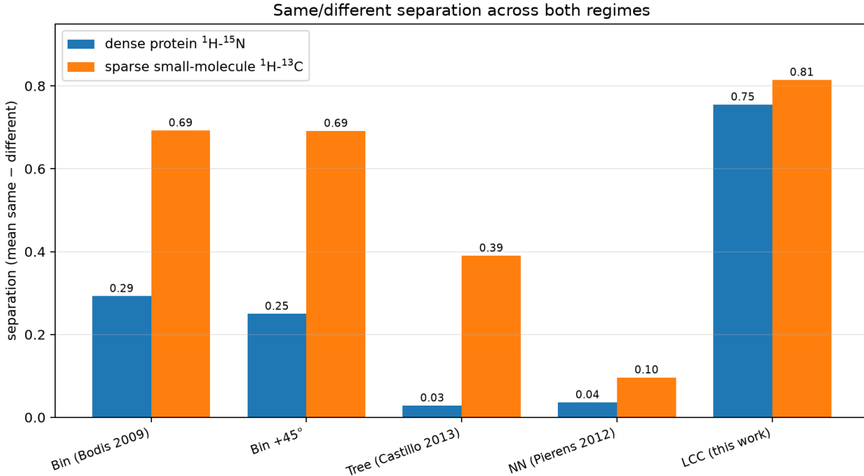
Figure 1: Figure 1. Same/different separation (mean same-class — mean different-class similarity) for all five methods on the two benchmarks: dense protein ^1\text{H} - ^{15}\text{N} (blue) and sparse small-molecule ^1\text{H} - ^{13}\text{C} (orange). LCC is the only method with a large separation in both regimes; the tree and nearest-neighbour methods saturate in both.
