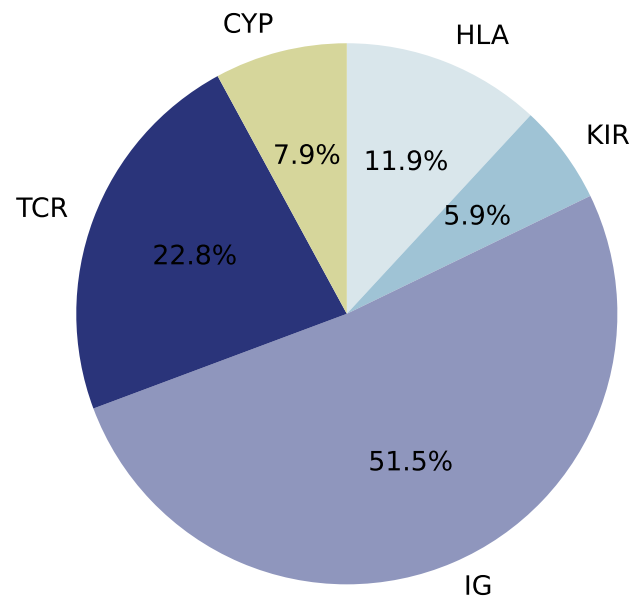
Community 1
