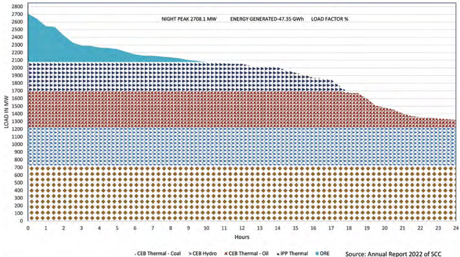
DAILY LOAD DURATION CURVE ON THE DAY OF MAXIMUM NIGHT PEAK - 2022-01-31 MONDAY
