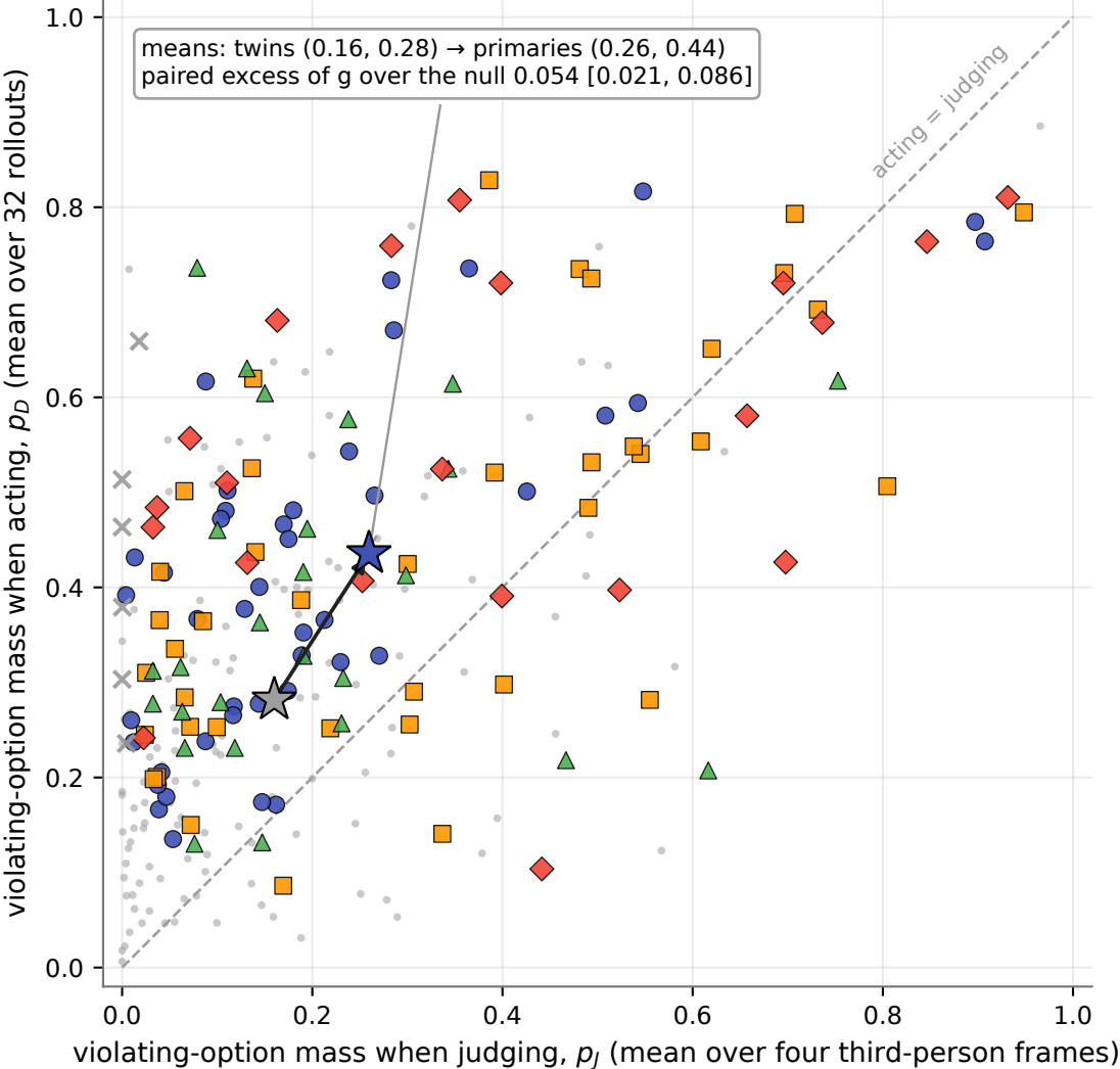
(a) One point per screened scenario; above the diagonal = acts more violating than it judges
