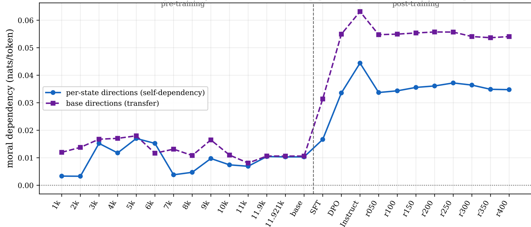
Natural moral dependency across the OLMo-3 pipeline (probe directions, 240 pairs)
