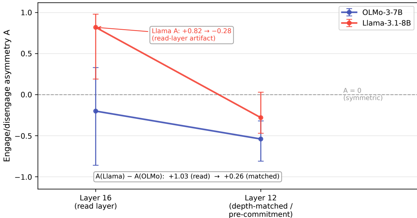
(a) Asymmetry A vs patch layer (read layer 16 to depth-matched 12)
