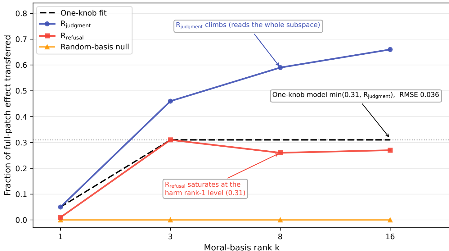
(a) Transfer fraction vs moral-basis rank k (nested interchange sweep)
