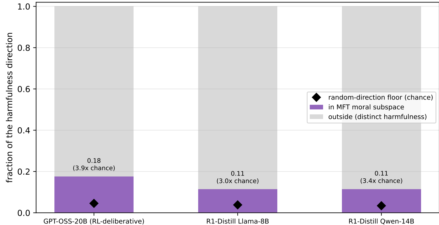
Harmfulness is largely distinct from moral foundations, with a small above-chance moral component
