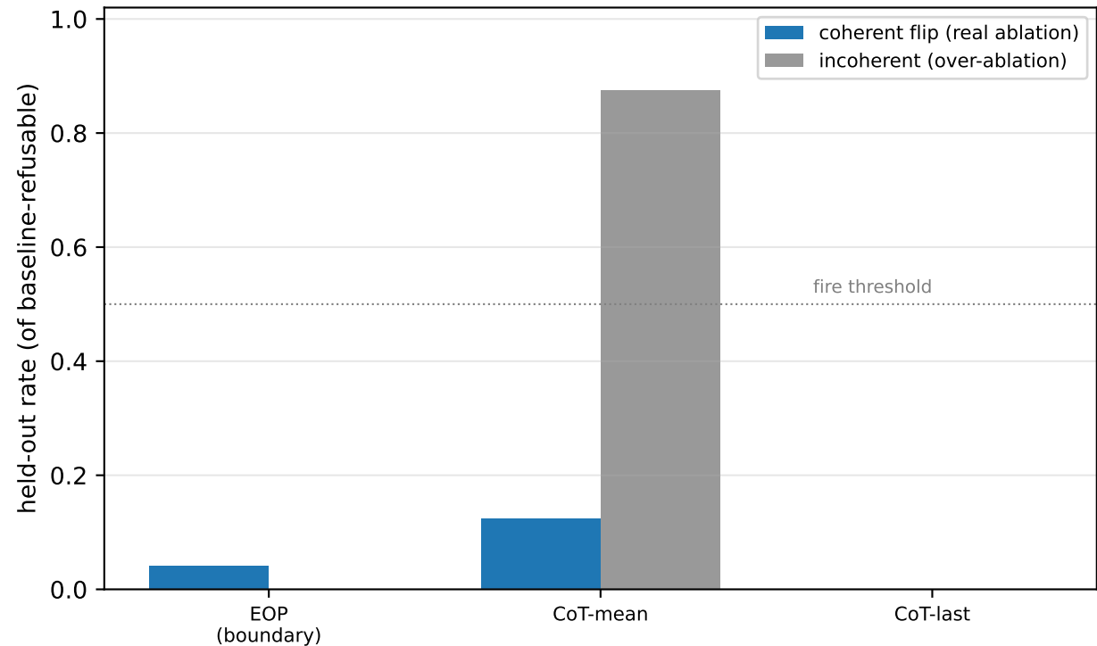
GPT-OSS refusal is distributed: no single direction cleanly ablates it
