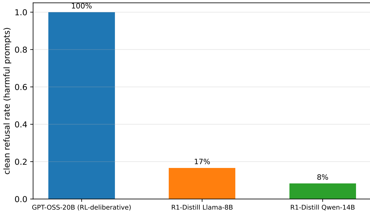
Behavioral contrast — confounded: R1 distillation degrades refusal (a lower bound; soft-refuse-by-reframe under-counted)
