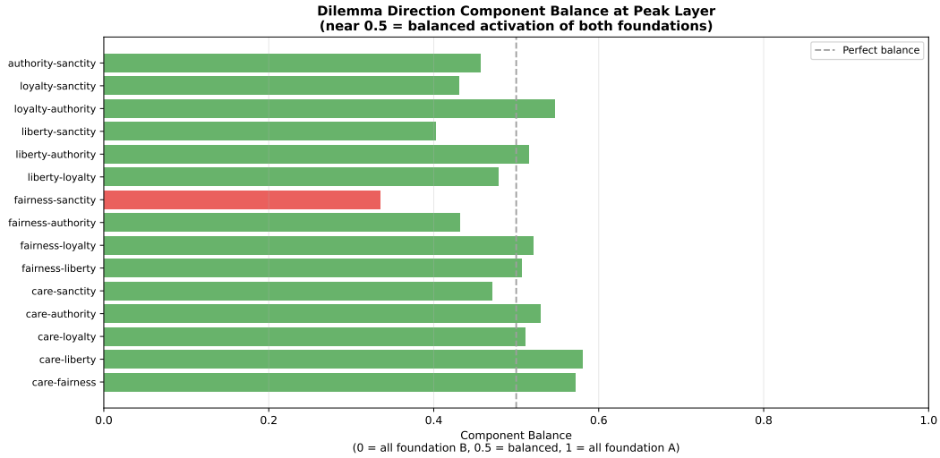
Figure 8: Component balance at each pair's peak subspace membership layer. Values near 0.5 (dashed line) indicate balanced contribution from both foundations. Fairness–sancity (red) is the only pair with substantial imbalance.
