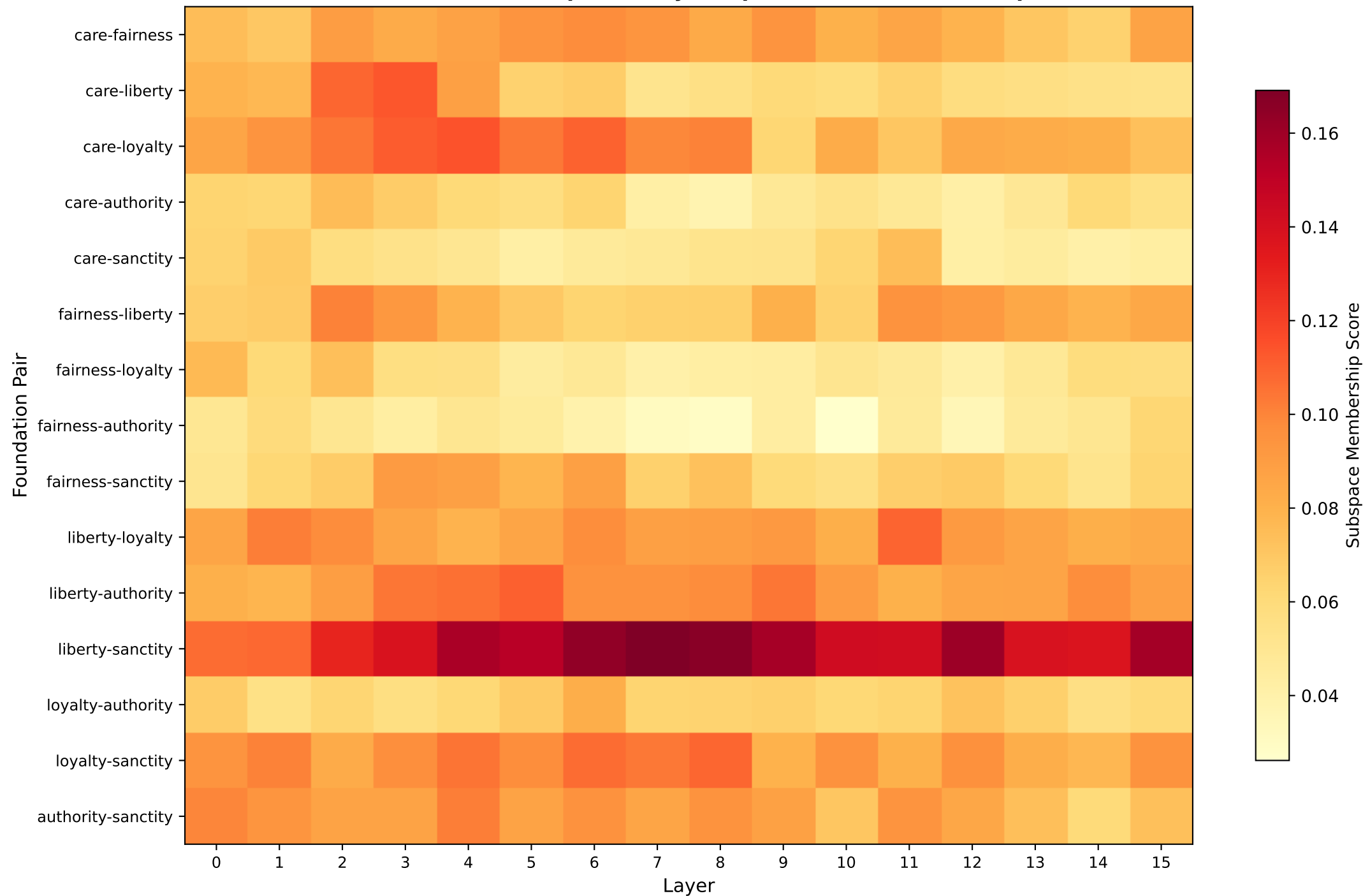
Dilemma Direction Subspace Membership (fraction of variance explained by component foundation subspace)
