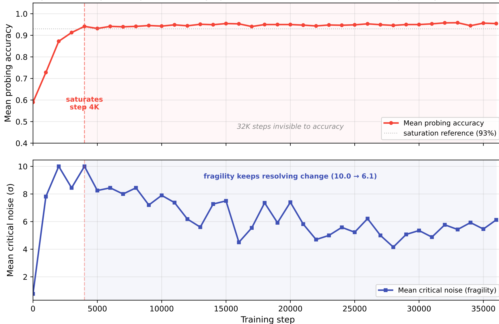
Figure 2: Probing accuracy saturates; fragility resolves --- allenai/OLMo-2-0425-1B-early-training
