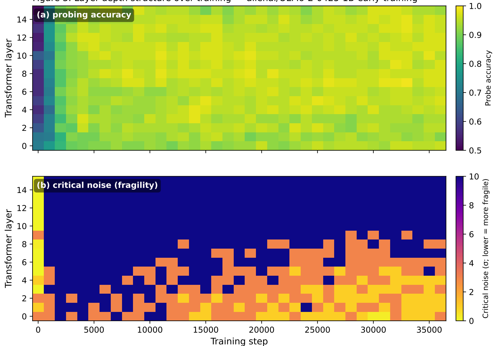
Figure 3: Layer-depth structure over training --- allenai/OLMo-2-0425-1B-early-training
