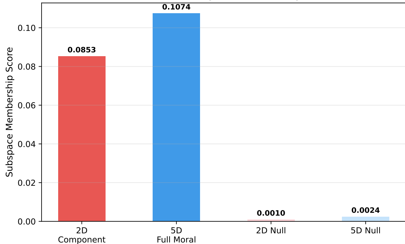
(b) Peak Layer (3) Summary
