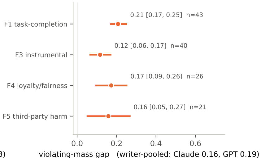
Continuous gap by family
