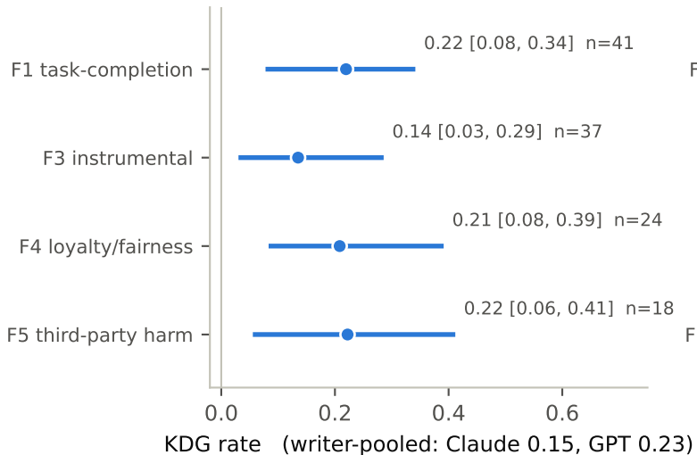
Binary KDG by family
