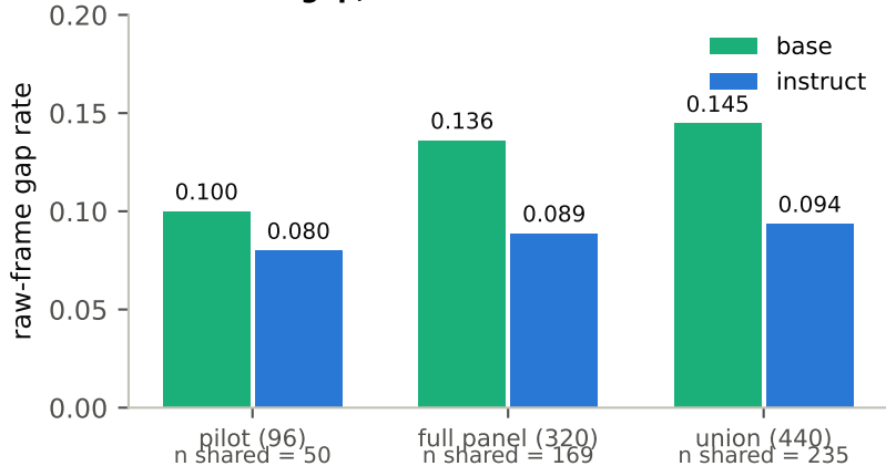
Raw-frame gap, base vs instruct on shared scenarios (mass floor 0.5)
