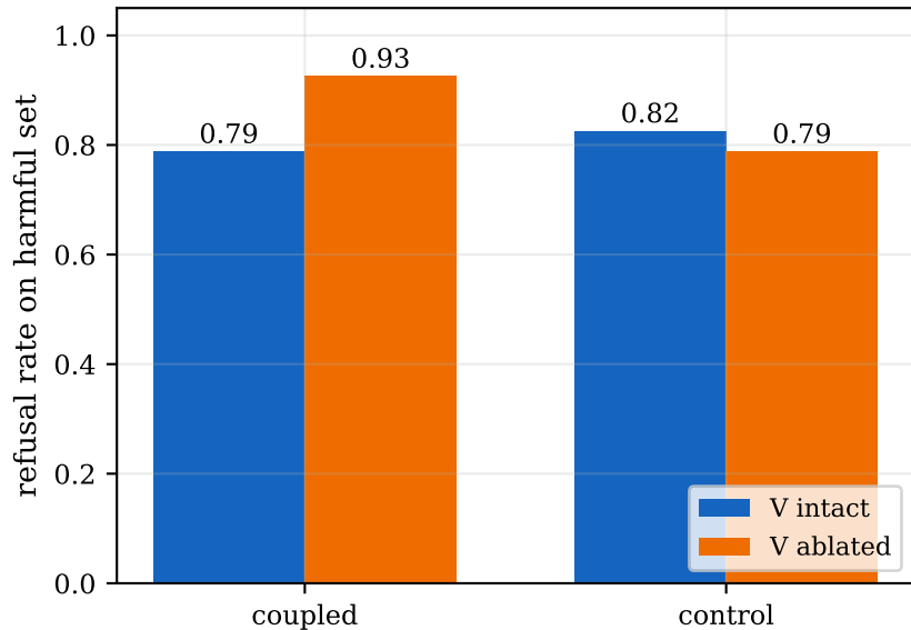
(b) Ablating V raises refusal, not removes it
