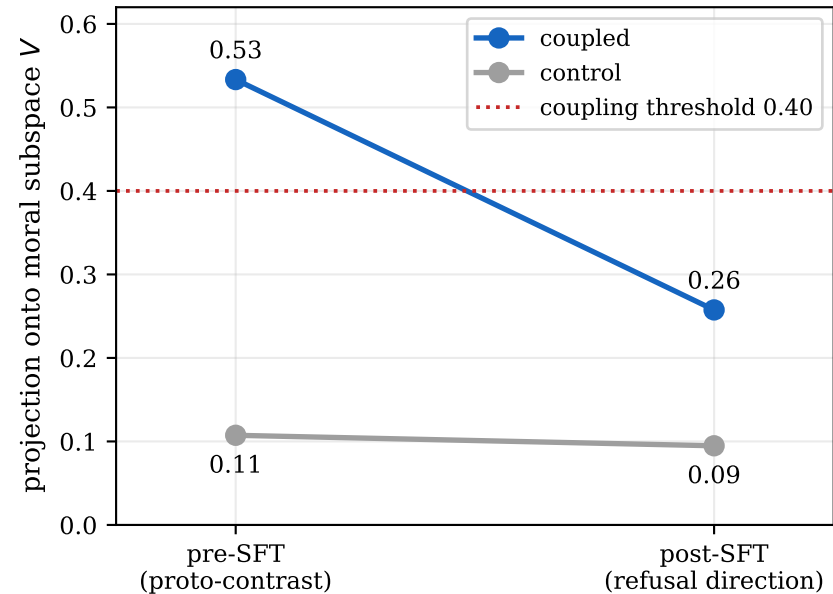
(a) Geometric coupling degrades through SFT
