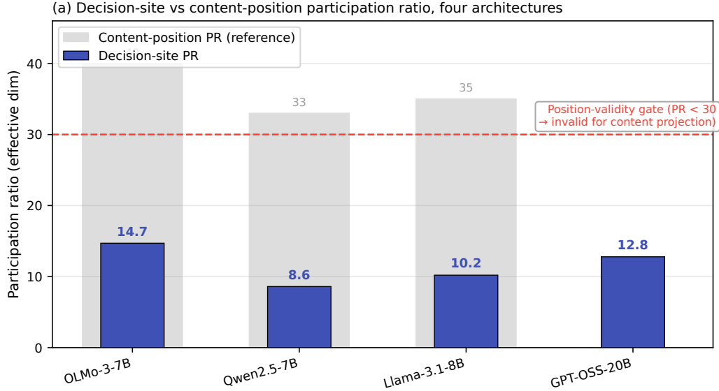
Figure 3: The decision-site participation ratio across four architectures: OLMo-3-7B-Instruct 14.7, Qwen2.5-7B 8.6, Llama-3.1-8B 10.2, and GPT-OSS-20B 12.79 (a 20B reasoning mixture-of-experts at its harmony decision token). All four fall below the participation-ratio 30 position-validity gate, while content positions at the same layers stay full-rank-healthy (above 40/33/35). The refusal decision lives in a 9-to-15 effective-dimensional control-token channel on every model tested.
