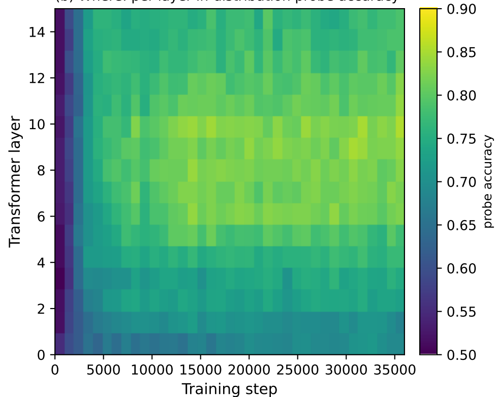
(b) Where: per-layer in-distribution probe accuracy
