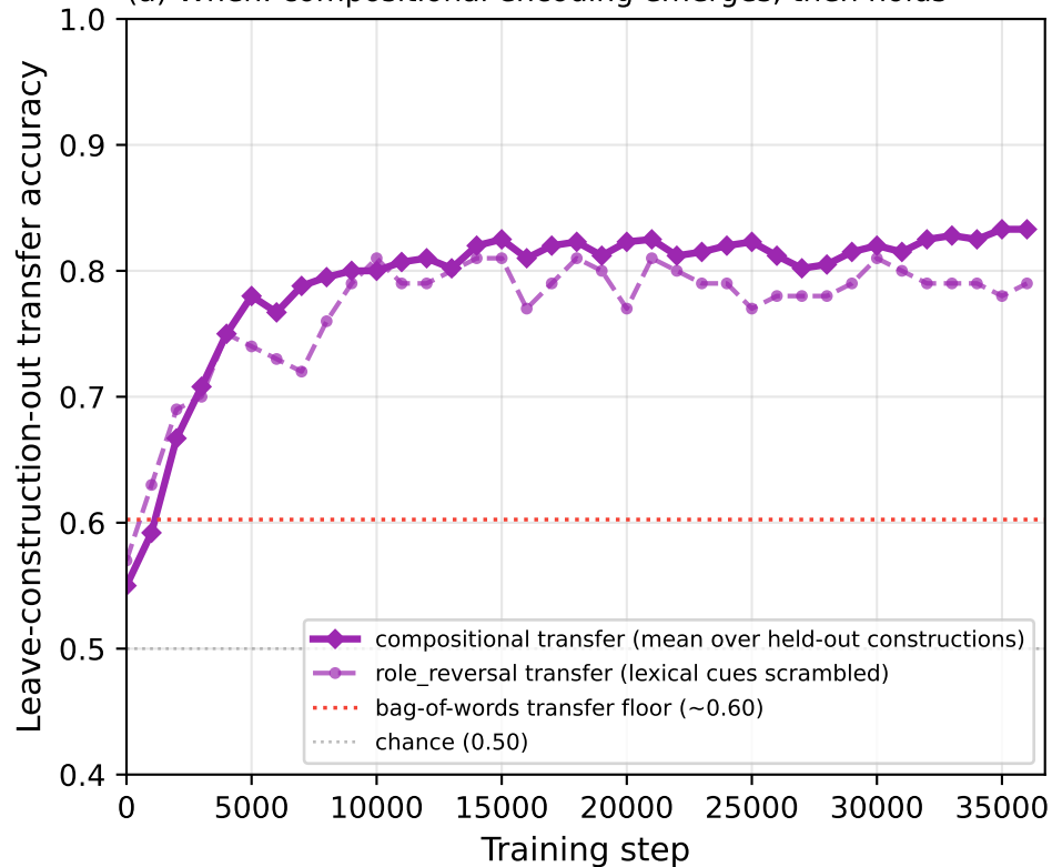
(a) When: compositional encoding emerges, then holds
