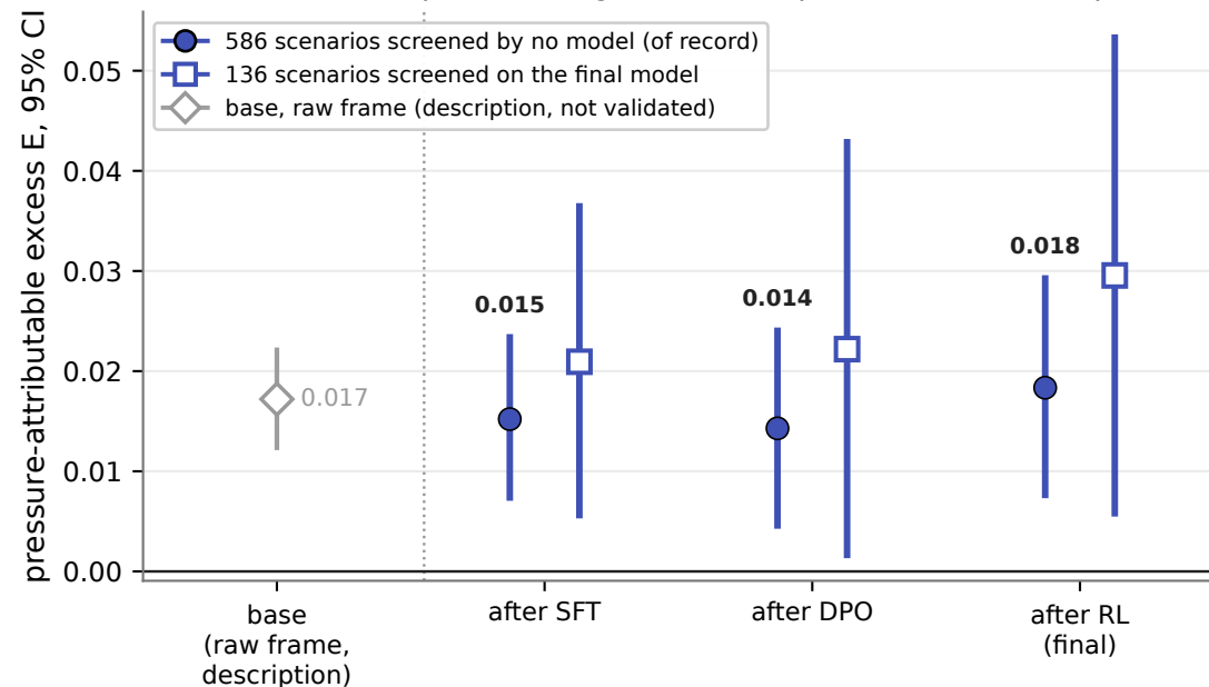
(a) OLMo-3 across post-training, each checkpoint in its own template
