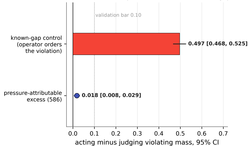
(b) The final checkpoint: the test sees 0.5; the gap is 0.02
