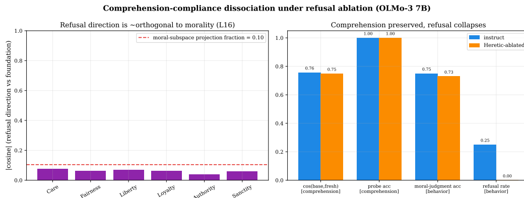
Figure 4: Left: the refusal direction is nearly orthogonal to every moral foundation ( |\cos| < 0.10 , below the moral-subspace projection fraction). Right: ablating the refusal direction leaves comprehension untouched (direction-transfer cosine and probe accuracy identical to Instruct) while the refusal rate collapses from 0.25 to 0.00; moral judgment accuracy is preserved.
