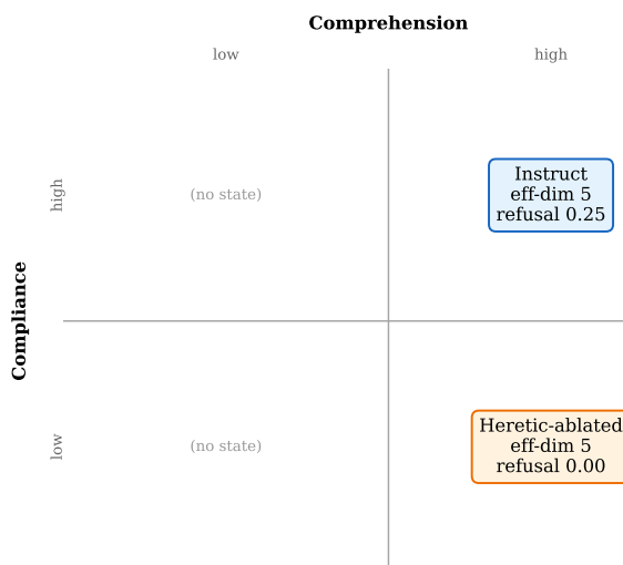
Figure 5: The dissociation matrix, populated. The low-comprehension column is empty: every OLMo-3 state has full comprehension (effective dimensionality 5). The two populated cells differ only in compliance (refusal rate on harmful requests): Instruct refuses, the refusal-ablated model does not.
