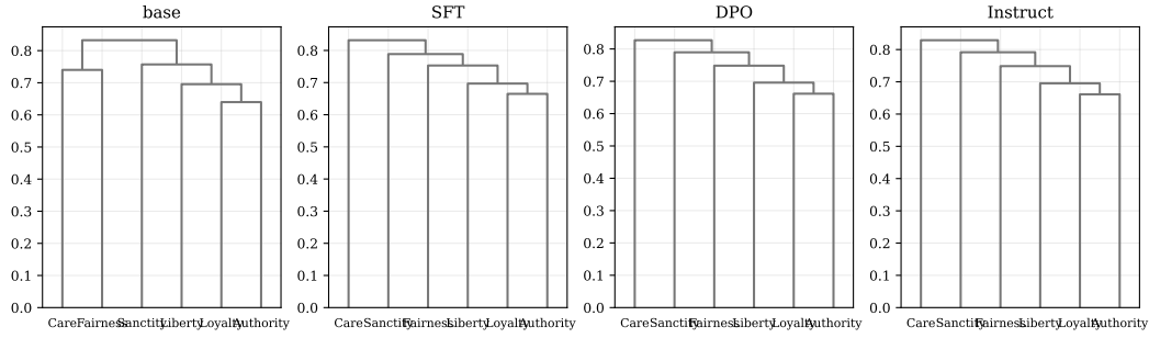
Figure 2: Foundation clustering (Ward linkage on 1 - \cos ) at base, SFT, DPO, and Instruct. The Loyalty–Authority binding pair persists across all stages. SFT mildly reorganizes the rest: Care shifts from pairing with Fairness (base) to an outlier, and Sanctity pairs with Fairness.
