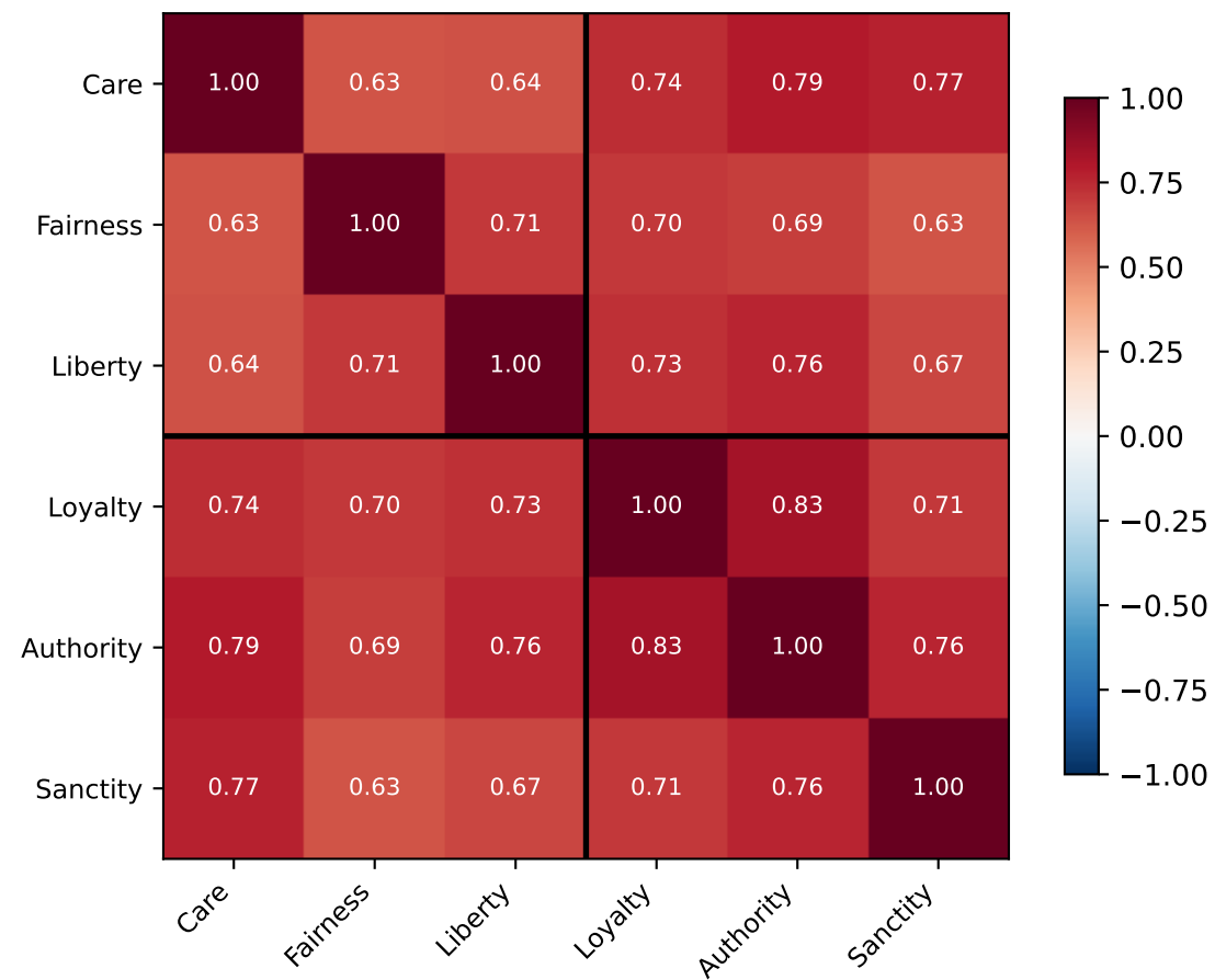
(a) MFV cosine (layer 12) mean = 0.718
