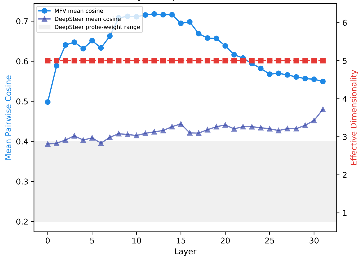
(b) Geometry vs depth (matched estimator)
