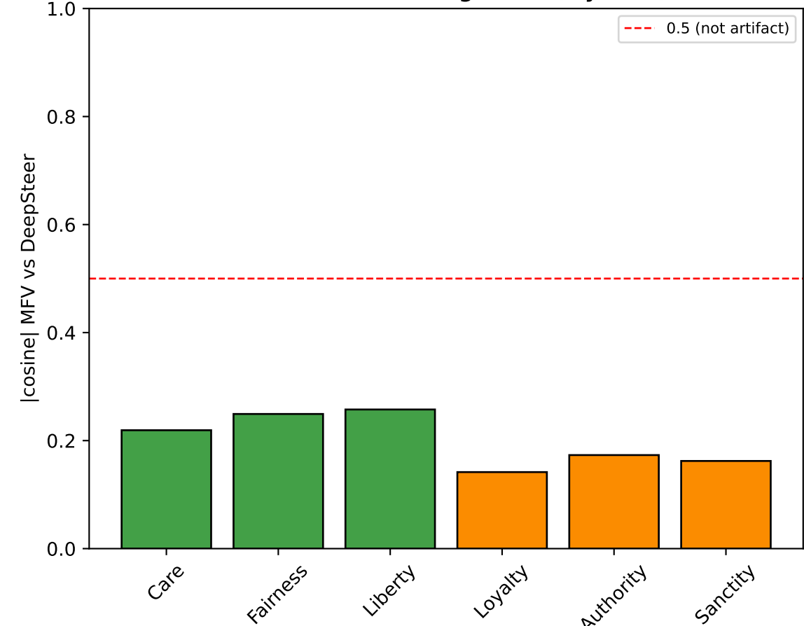
(c) Cross-dataset alignment (layer 12)
