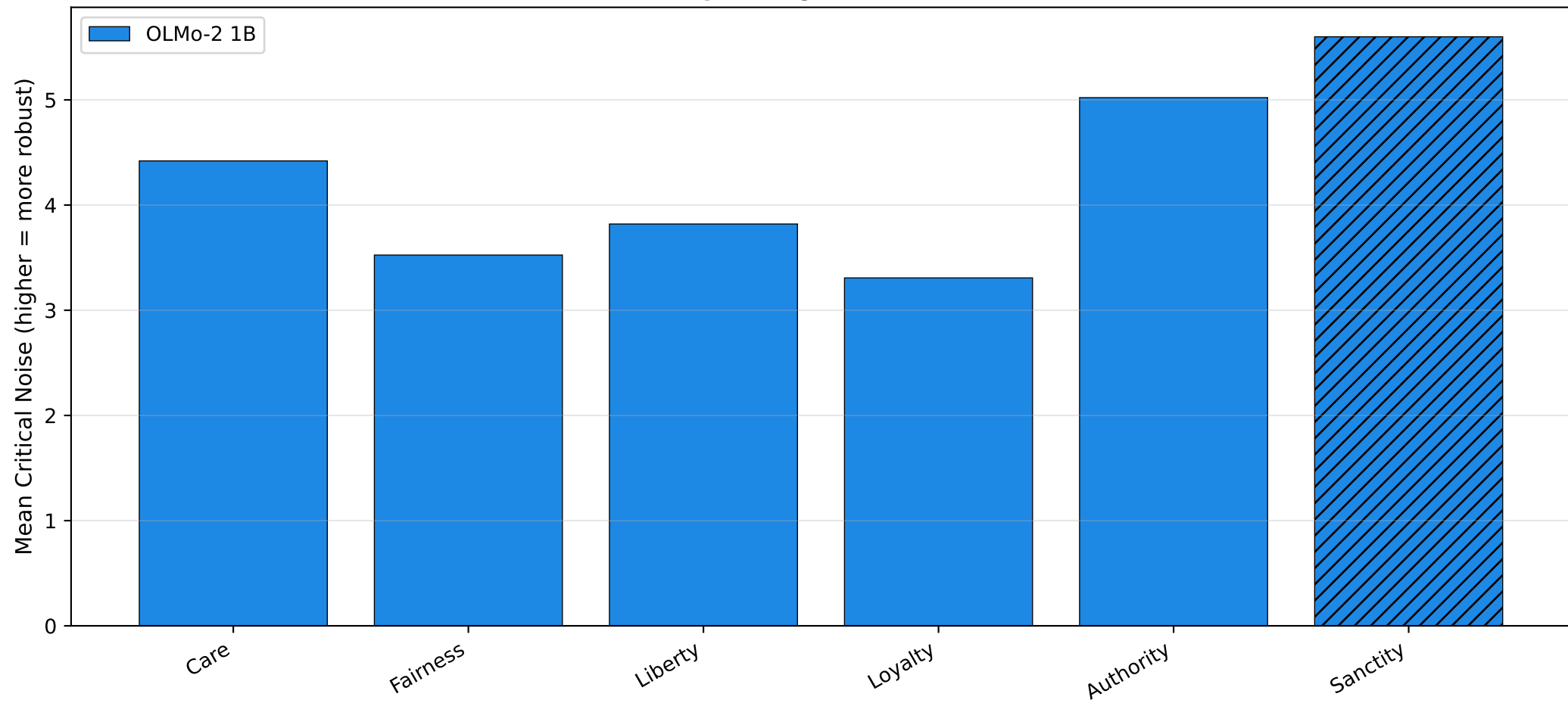
Per-Foundation Fragility Across Scale (sanctity hatched) [7B pending RunPod run]
