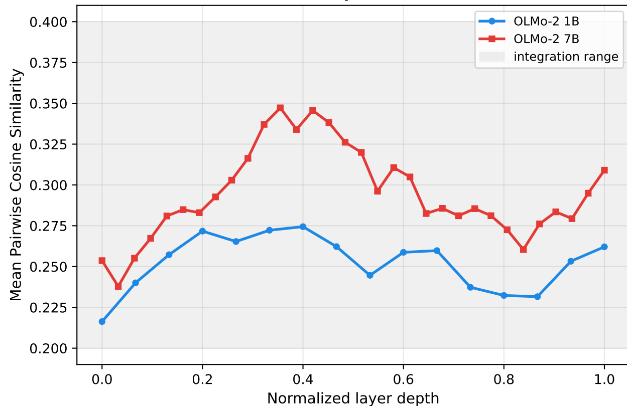
(a) Collapse Metric
