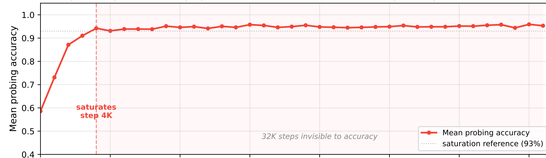
Probing accuracy saturates; fragility resolves --- allenai/OLMo-2-0425-1B-early-training
