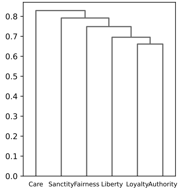
olmo3_instruct_final (L16)
