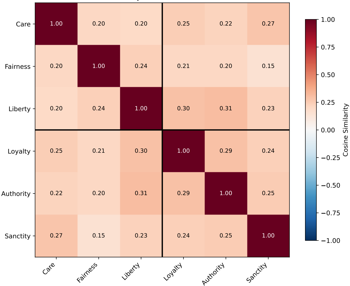
Foundation Probe Direction Cosine Similarity (Layer 1) Mean pairwise = 0.2378
