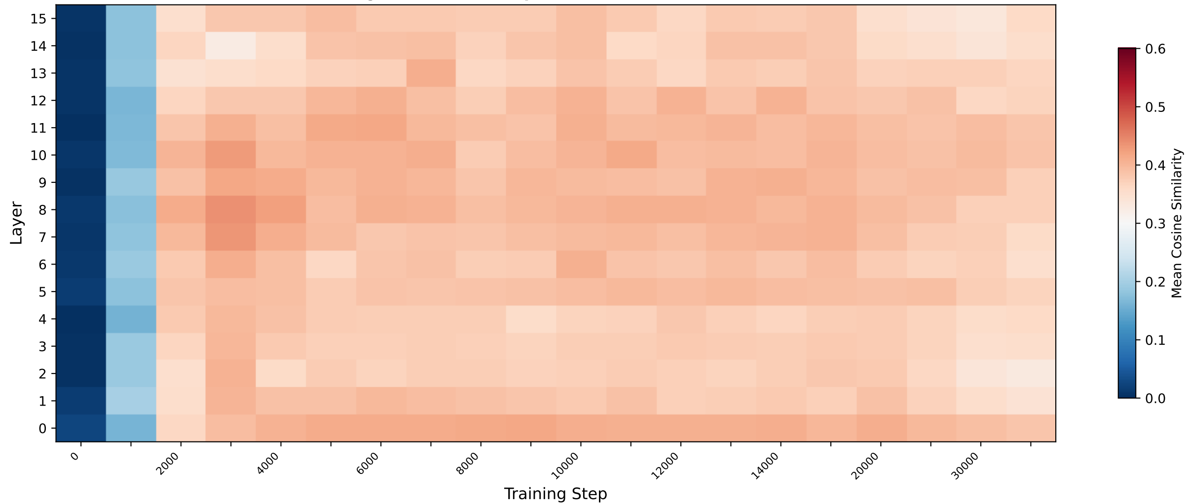
Mean Pairwise Cosine Similarity Across Training (higher = more collapsed framework directions)
